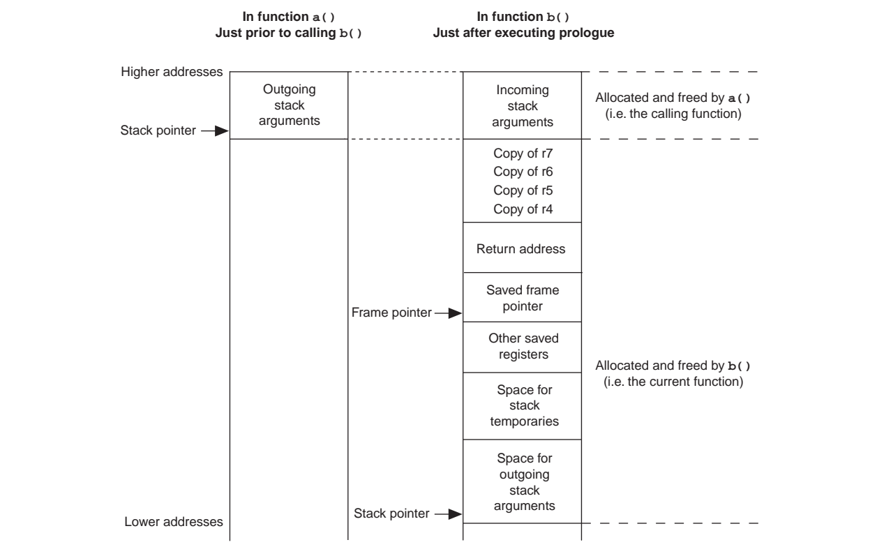
Figure 7-3. Stack Frame Using Variable Arguments
